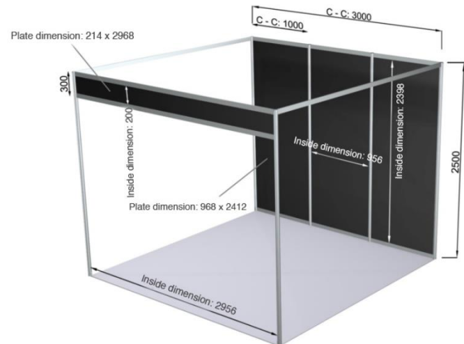
Example of 3 m x 3 m booth
